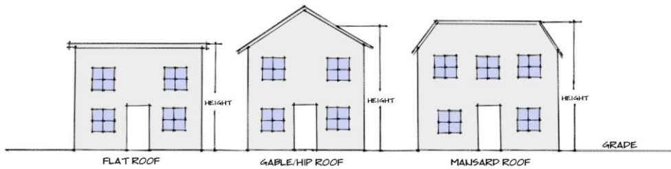
Figure 7-5: Building Height
