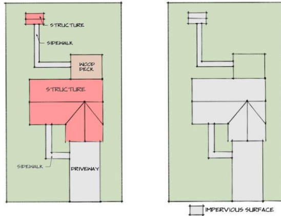
Figure 7-4: Lot Coverage
