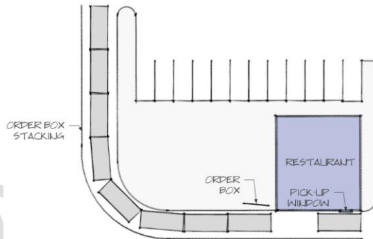
Figure 8-3: Stacking Spaces
