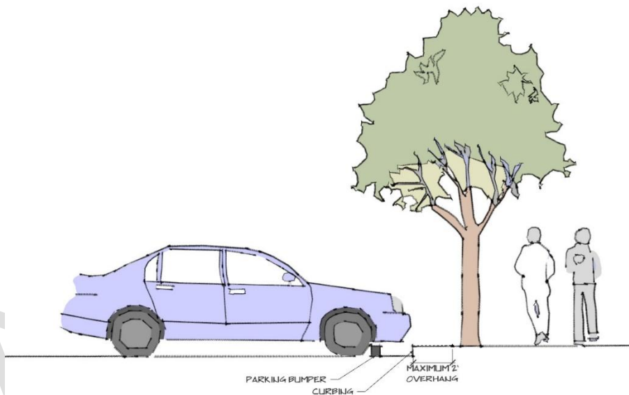
Figure 8-2: Protective Curbing
